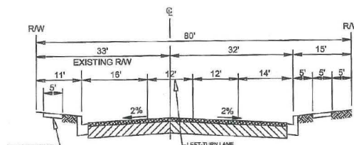
MENLO AVENUE (TRANSITION TO CAWSTON AVE.) TYPICAL SECTION E-E N.T.S.
