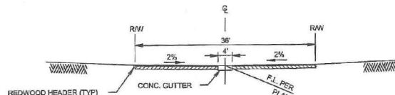
TYPICAL SECTION C-C N.T.S. PRIVATE DRIVES
