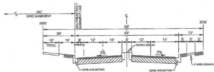
MENLO AVENUE W/ RAISED MEDIAN TYPICAL SECTION D-D N.T.S. (STD. NO. 102-A MODIFIED)
