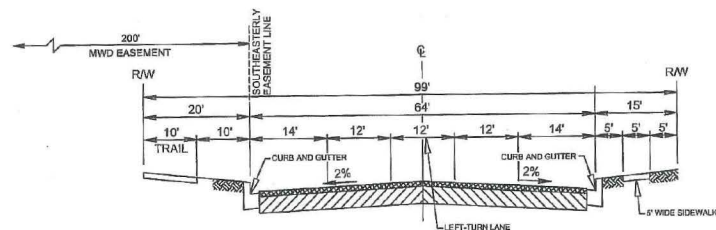
MENLO AVENUE W/ RAISED MEDIAN TYPICAL SECTION D-D N.T.S. (STD. NO. 102-A MODIFIED)
